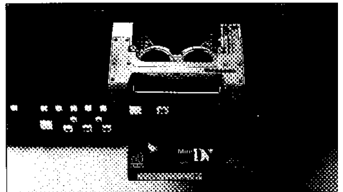
Playback with Cassette Adaptor, AJ-CS750 in DVCPRO/Studio VT.
